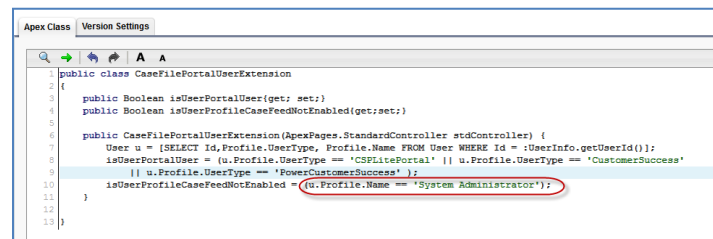
Figure 1 CaseFilePortalUserExtension Code
